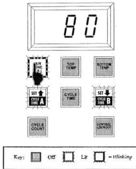
Figure 8-1 Setting Air Line Pressure Lockout
