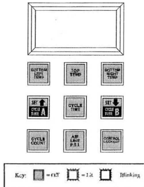
Figure 4-1 DES-42 Control Panel with Buttons Off
